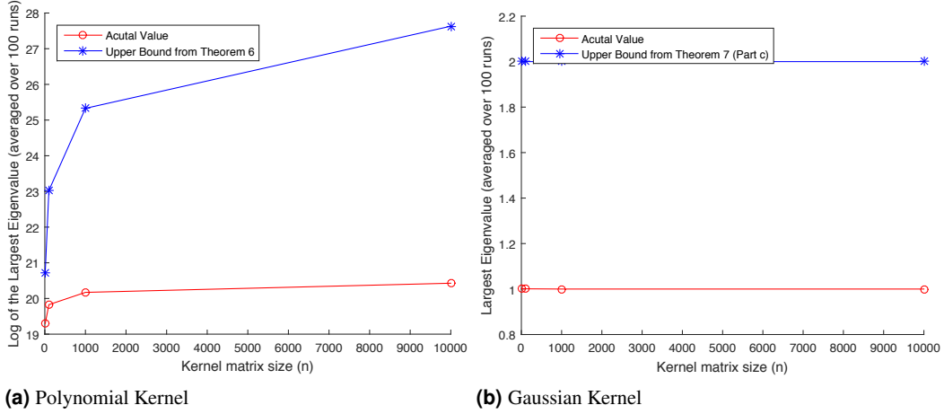
■ Figure 1 Largest eigenvalue distribution for random kernel matrices constructed with a polynomial kernel (left plot) and a Gaussian kernel (right plot). The actual value plots are constructed by averaging over 100 runs, and in each run we draw n independent standard Gaussian vectors in d = 100 dimensions. The predicted values are computed from bounds in Theorems 6 and 7 (Part c). The kernel matrix size n is varied from 10 to 10000 in multiples of 10. For the polynomial kernel, we set a = 1 , b = 1 , and p = 4 , and for the Gaussian kernel a = 3 \log(n)/d . Note that our upper bounds are fairly close to the actual results. For the Gaussian kernel, the actual values are very close to 1.
